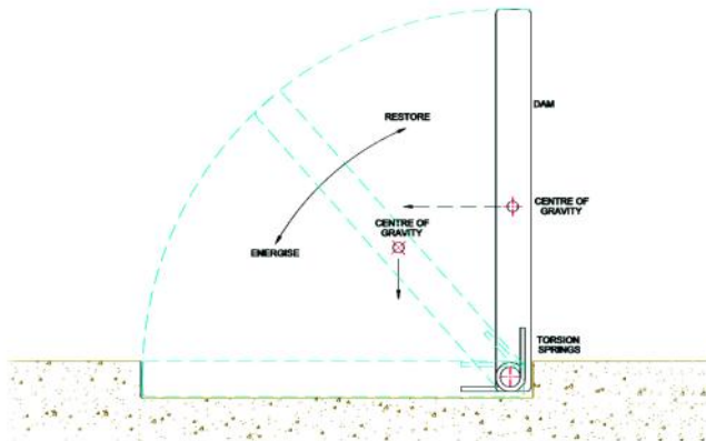
Manually Assisted Spring-Powered Flood Defence
